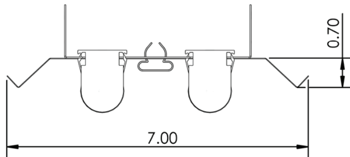
END VIEW
